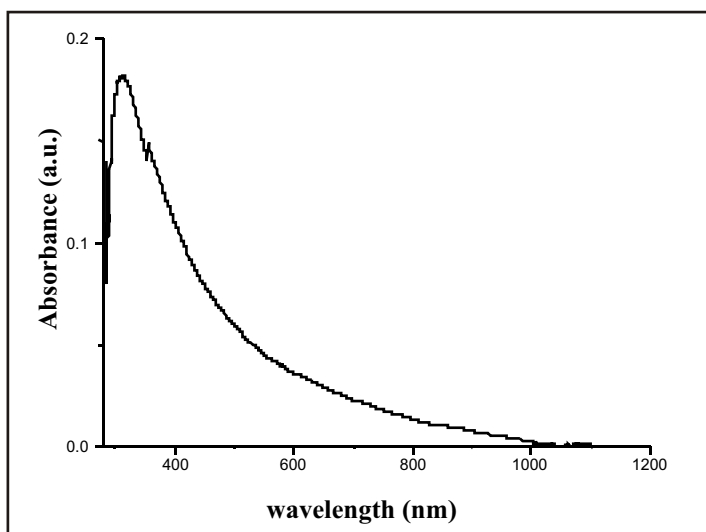
Figure 6: Ultraviolet-visible Spectrum of \text{TiO}_2/\text{ZnO} Nanocomposite Prepared at 180^\circ\text{C} for 12hrs
