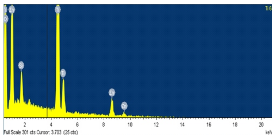
Figure 2A: Energy Dispersive Spectrum of a Representative Grain
