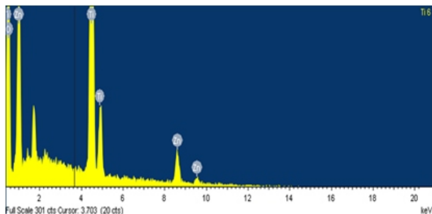
Figure 2B: Energy Dispersive X-ray Spectra of Representative Grains
