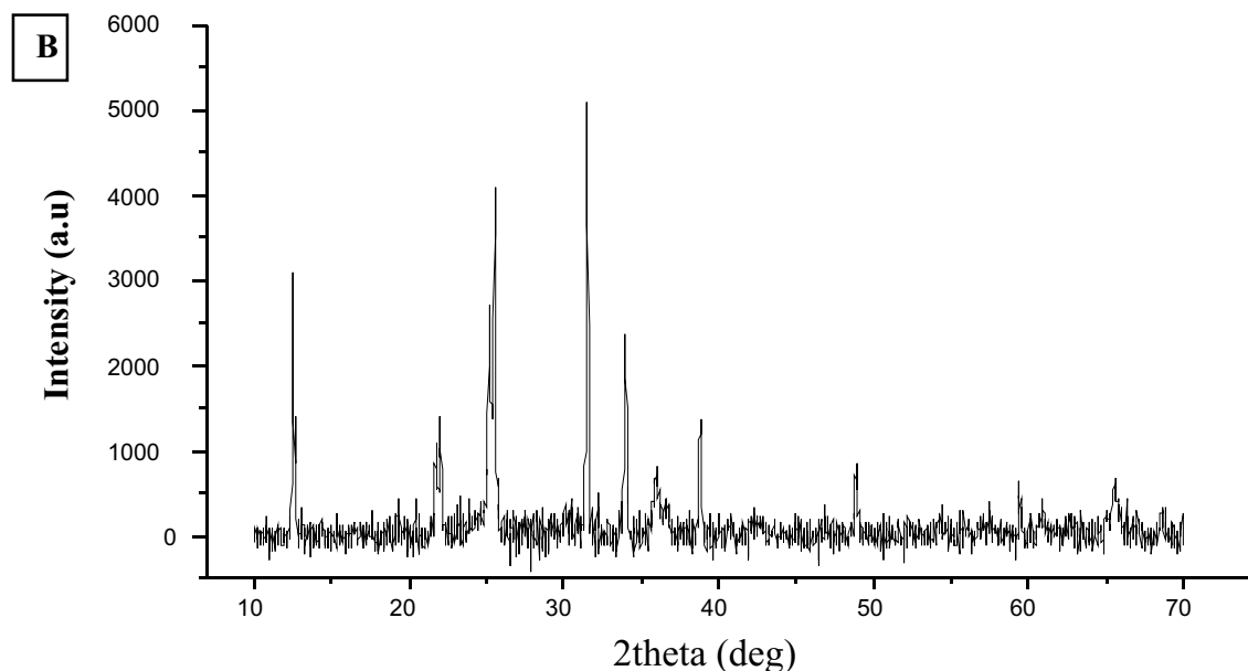
Figure 3B: XRD Spectrum of \text{TiO}_2\text{-ZnO} at 180^\circ\text{C}
