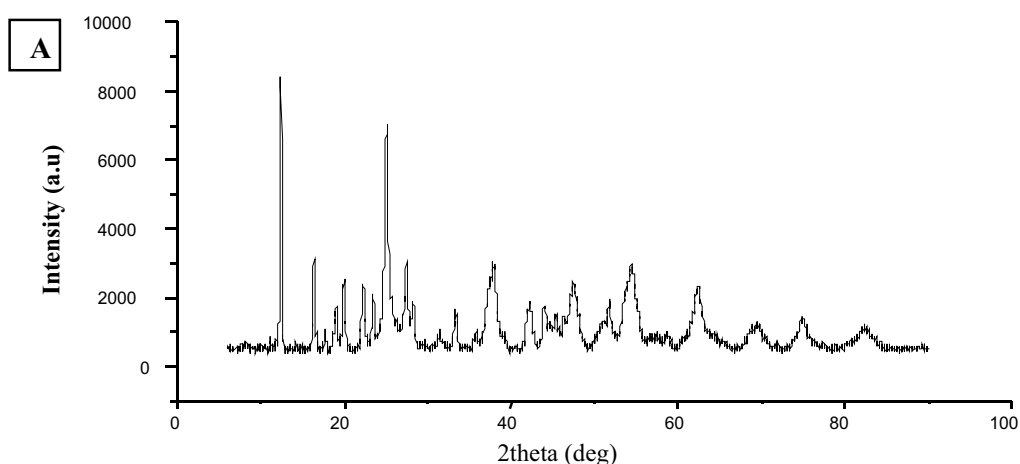
Figure 3A: XRD Spectrum of \text{TiO}_2 -Zn(OOCCH 3 ) 2 at 90^\circ\text{C} .
