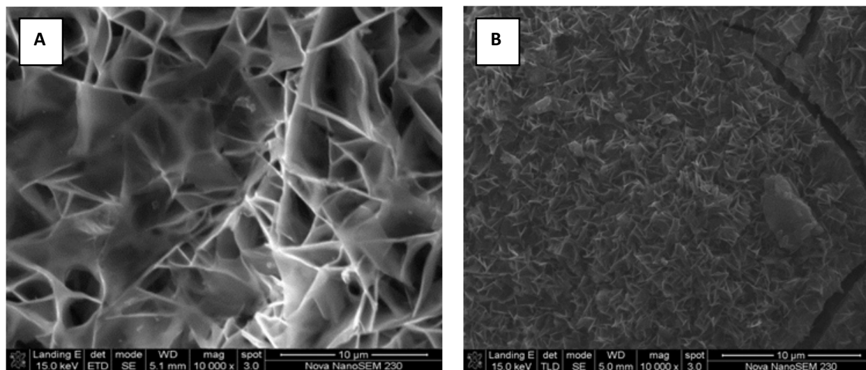
Figure 4: SEM Images of \text{TiO}_2/\text{Zn}(\text{OOCCH}_3)_2 Mixtures Prepared at 90^\circ\text{C} at Low Magnification (A) 6hrs (B) 12hrs
