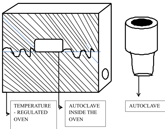
Figure 1: Schematic Representation of the Hydrothermal Set-up (Inset: Autoclave Diagram)
