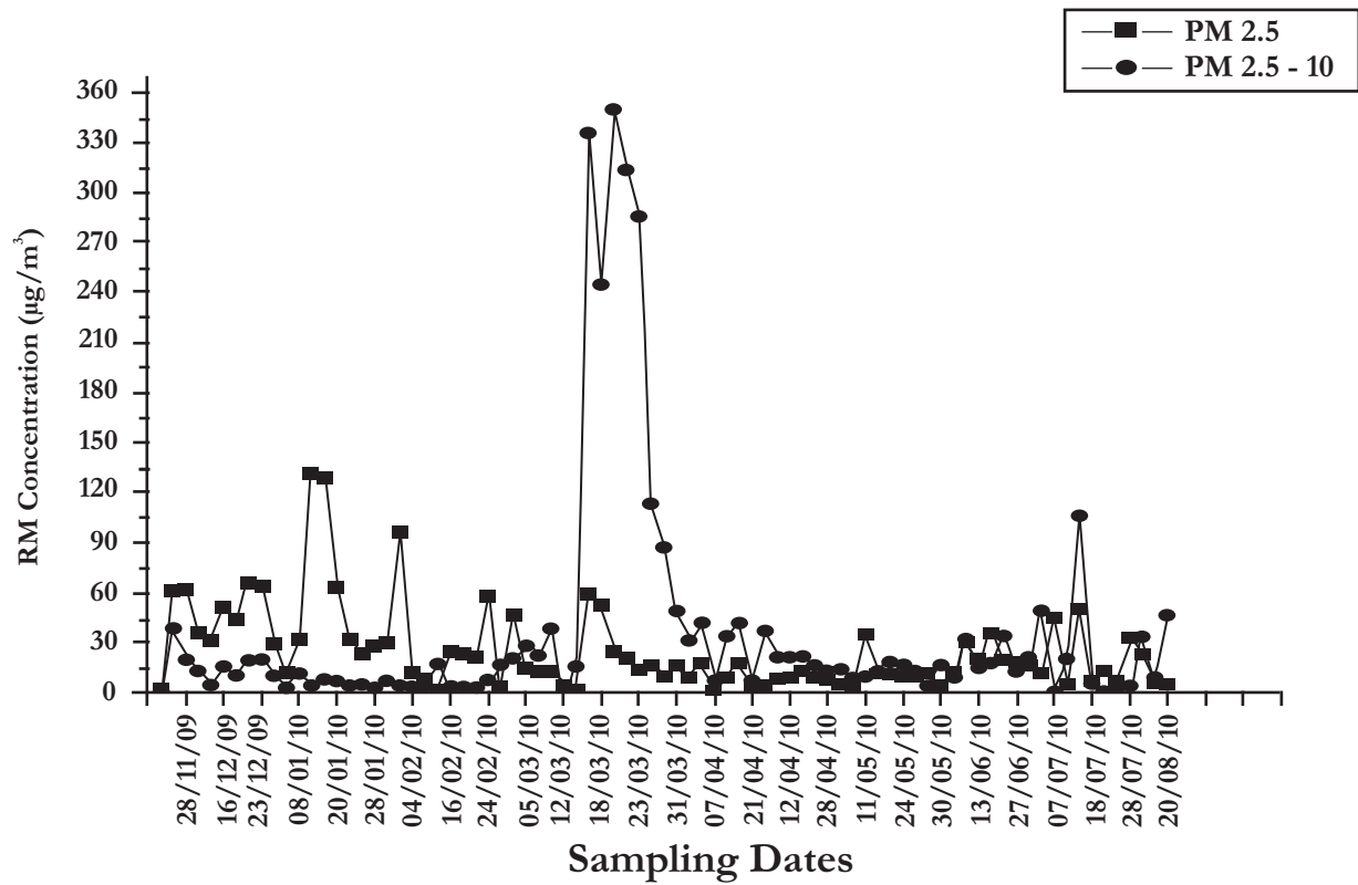
Figure 2: Daily Variation of Concentration of Particulate Matter in \mu\text{g}/\text{m}^3
