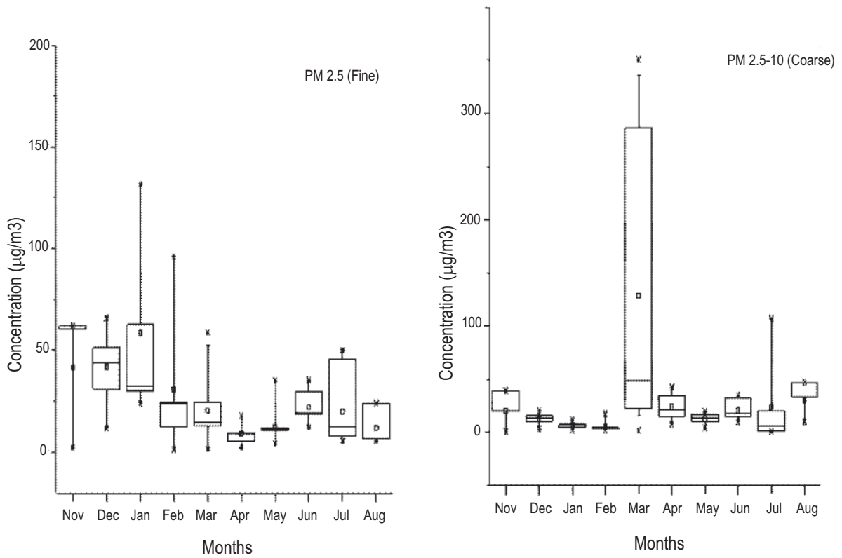
Figure 3a and b: Box-Whisker Plot for monthly mass concentration at top of \text{PM}_{2.5} and \text{PM}_{2.5-10} .
