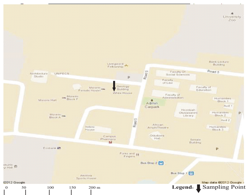
Figure 1: Google map of the Obafemi Awolowo University Campus, Ile-Ife, Nigeria showing the sampling point.
