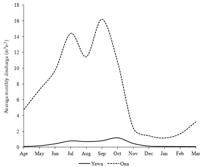
Fig. 2: Mean Monthly Flow of Ona and Yewa Rivers from 1988 – 1997
