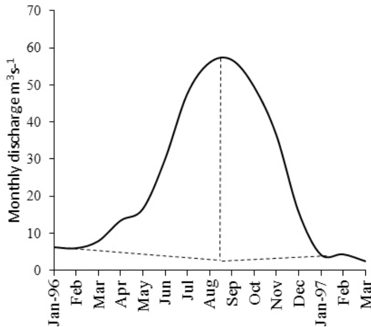
Figure 3: Hydrograph Separation Technique (Watson and Burnett, 1995)
