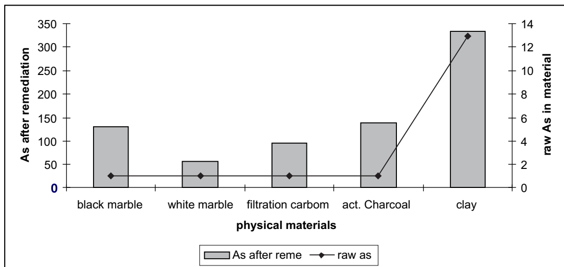
Figure 3. Statistical Plot of Bar Chat of As mg/L Concentrations in the Water of Geo-materials after Experiment in the Filtration Method
